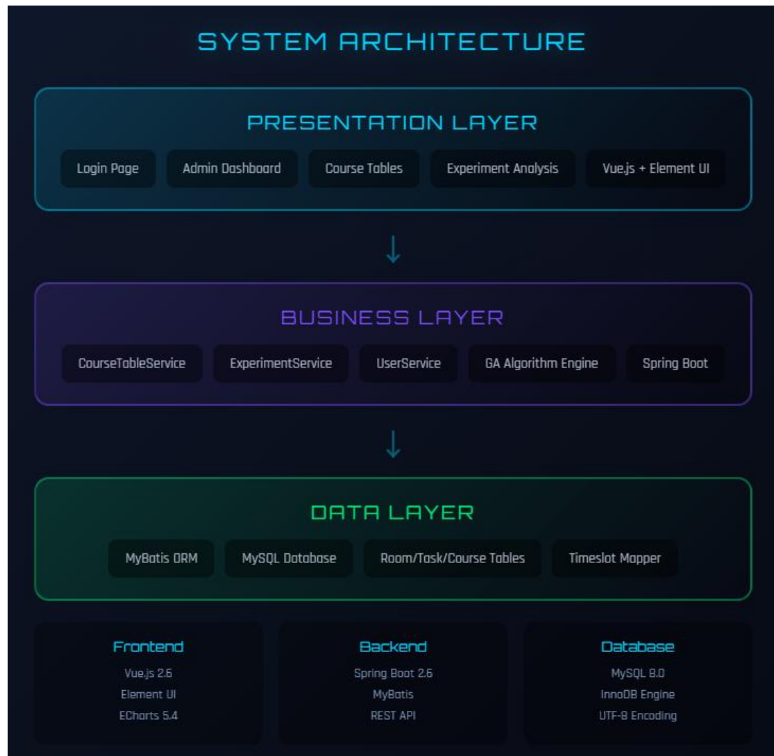
Figure 5.1: Three-Tier Architecture
