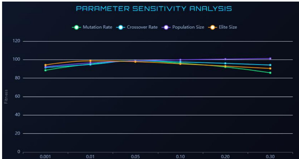
Figure 6.4: Parameter Sensitivity Analysis
