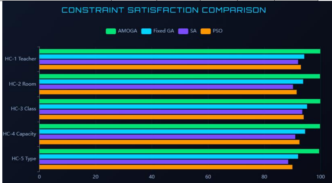
Figure 6.2: Constraint Satisfaction Comparison
