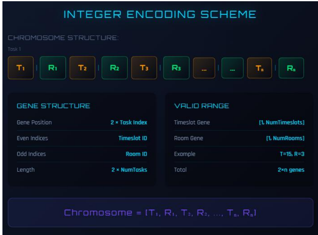
Figure 4.2: Chromosome Encoding Structure
