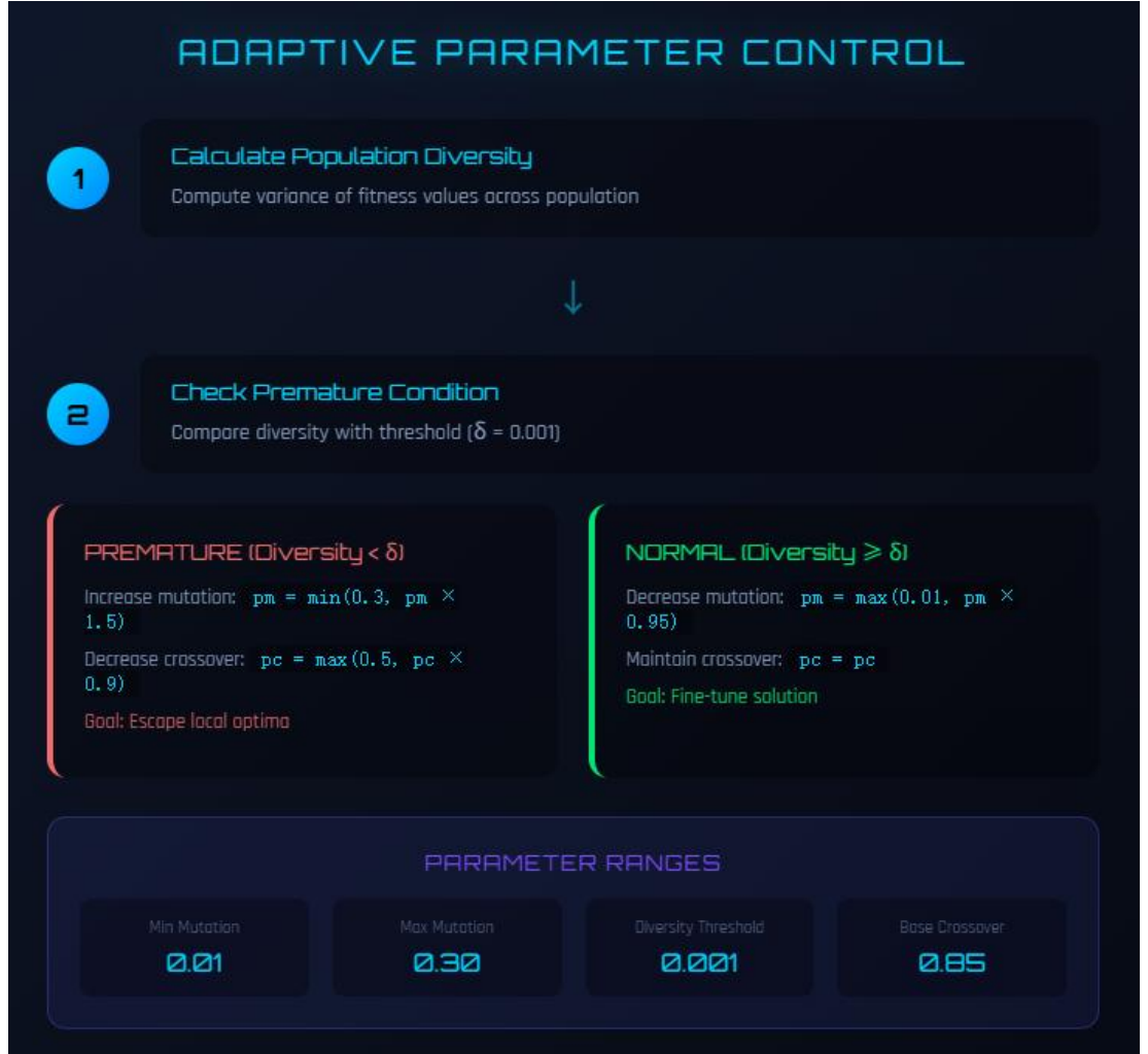
Figure 4.6: Adaptive Parameter Adjustment Mechanism
